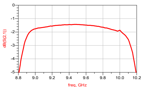
Insertion Loss VS Frequency (T A =25°C)
