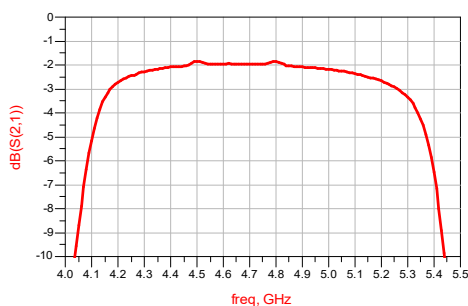
Insertion Loss VS Frequency (T A =25°C)
