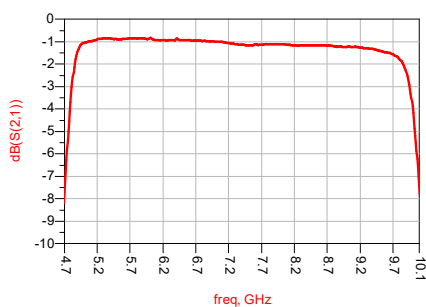
Insertion Loss VS Frequency (T A =25°C)
