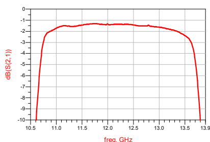
Insertion Loss VS Frequency ( T_A = 25^\circ\text{C} )
