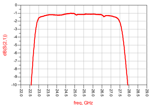
Insertion Loss VS Frequency (T A =25°C)
