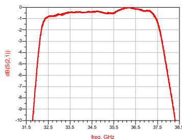
Insertion Loss VS Frequency (T A =25°C)
