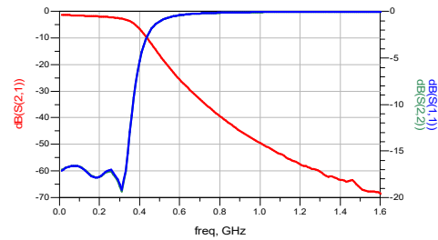
Broadband Insertion Loss VS Frequency ( T_A=25^\circ\text{C} )
