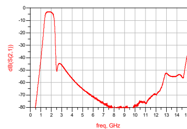
Broadband Insertion Loss VS Frequency ( T_A=25^\circ\text{C} )
