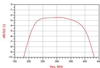
Insertion Loss VS Frequency (T A =25°C)
