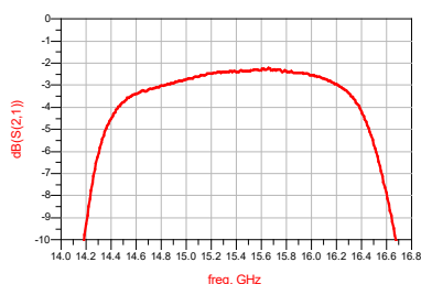
Insertion Loss VS Frequency (T A =25°C)
