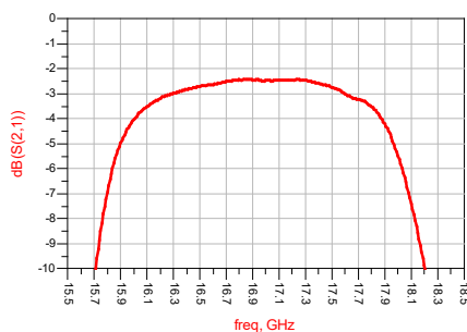
Insertion Loss VS Frequency ( T_A=25^\circ\text{C} )
