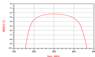
Insertion Loss VS Frequency (T A =25°C)
