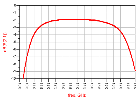
Insertion Loss VS Frequency (T A =25°C)
