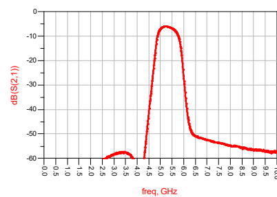
Broadband Insertion Loss VS Frequency ( T_A=25^\circ\text{C} )
