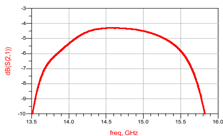
Insertion Loss VS Frequency (T A =25°C)
