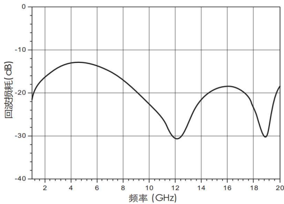
Coupling Output Return Loss
