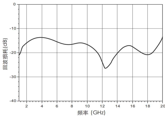
Input Return Loss vs. Freq
