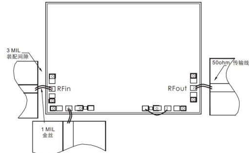
Application (Chip right side couple output)
