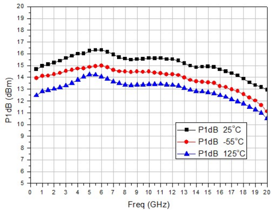
P1dB vs. Freq
