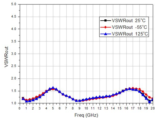
Output VSWR vs. Freq
