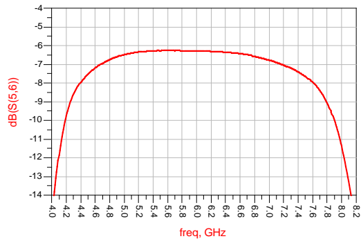
Pass band 5 Insertion Loss VS Frequency ( T_A=25^\circ\text{C} )
