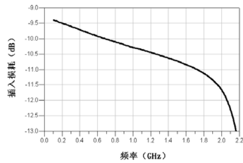
Pass band 5 Insertion Loss VS Frequency ( T_A=25^\circ\text{C} )
