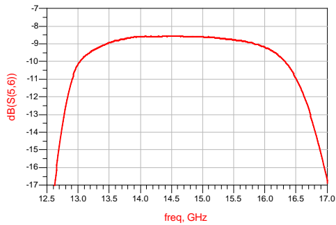
Pass band 3 Insertion Loss VS Frequency ( T_A=25^\circ\text{C} )
