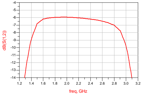
Pass band 1 Insertion Loss VS Frequency ( T_A=25^\circ\text{C} )
