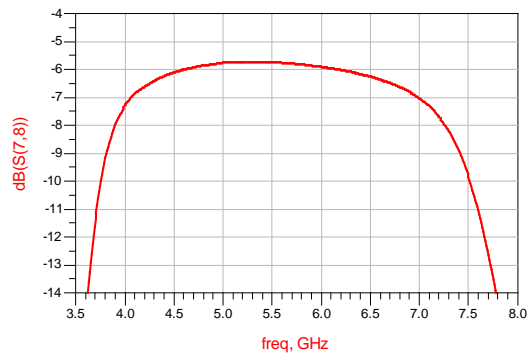
Pass band 6 Insertion Loss VS Frequency ( T_A=25^\circ\text{C} )
