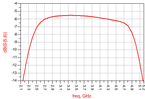
Pass band 3 Insertion Loss VS Frequency ( T_A=25^\circ\text{C} )
