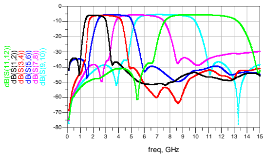
Insertion Loss VS Frequency ( T_A=25^\circ\text{C} )
