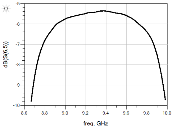
Insertion Loss VS Frequency ( T_A=25^\circ\text{C} )
