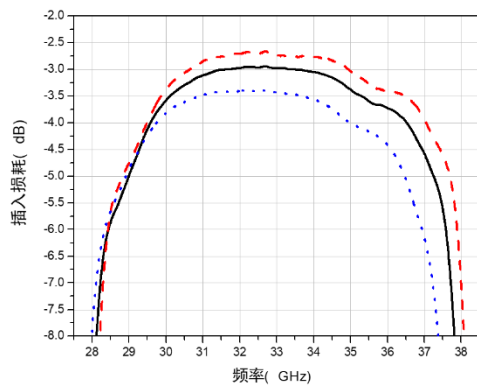
Insertion Loss VS Frequency ( T_A=25^{\circ}\text{C} )
