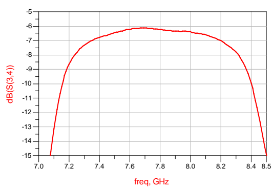
Pass band 2 Insertion Loss VS Frequency ( T_A=25^\circ\text{C} )
