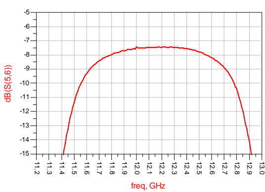
Pass band 3 Insertion Loss VS Frequency ( T_A=25^\circ\text{C} )
