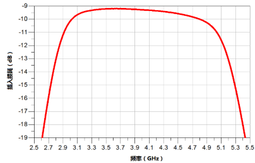
Pass band 5 Insertion Loss VS Frequency ( T_A=25^\circ\text{C} )
