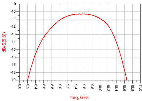
Pass band 5 Insertion Loss VS Frequency ( T_A=25^\circ\text{C} )
