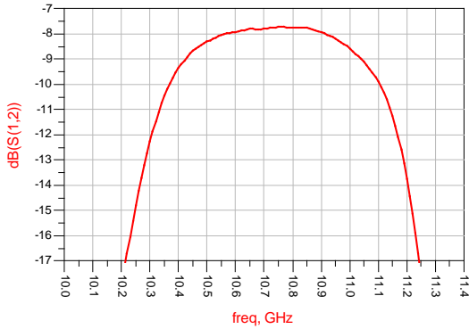
Pass band 3 Insertion Loss VS Frequency ( T_A=25^\circ\text{C} )
