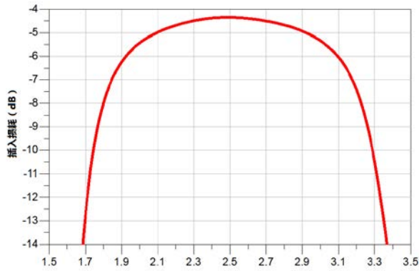
Pass band 1 Insertion Loss VS Frequency ( T_A=25^\circ\text{C} )
