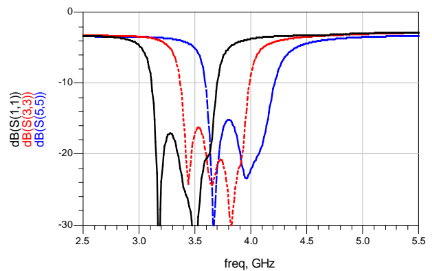
Return Loss VS Frequency ( T_A=25^\circ\text{C} )
