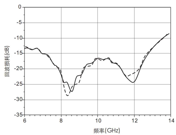
Attenuation state Input Return loss vs. Freq
