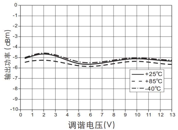
RFOUT/2 Output Power vs. Tuning Voltage Vcc=+5V
