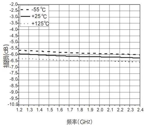
Insertion loss vs. Freq
