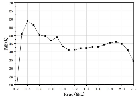
PAE @ 48V
