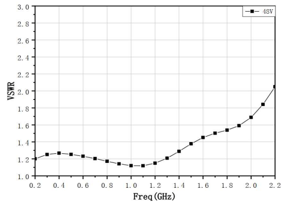
VSWRin @ 48V
