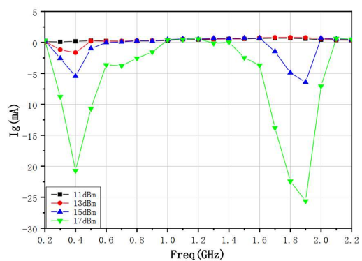
Gate Current vs. Different Pin
