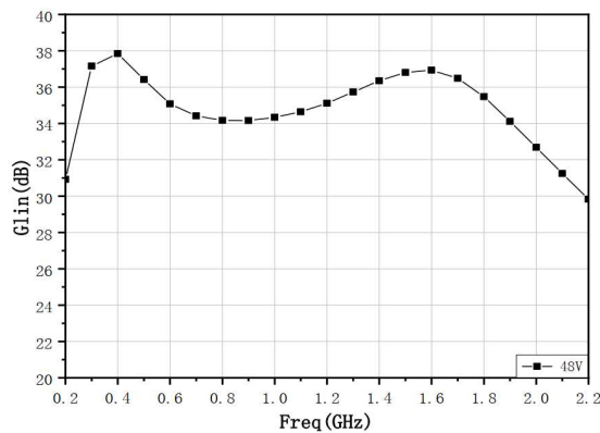
Small Signal Gain @48V
