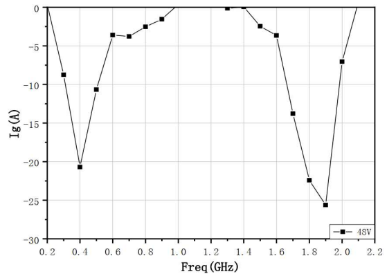
Gate Current @ 48V
