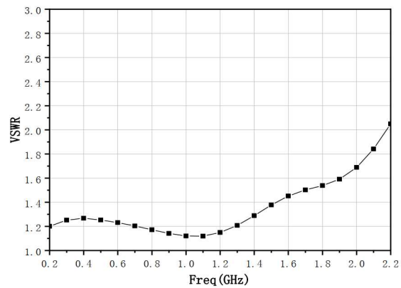
VSWRin @ 48V
