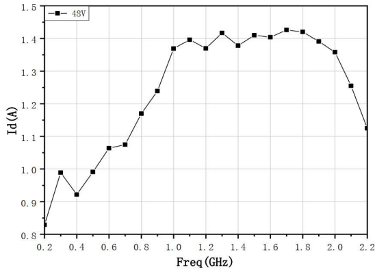
Drain Current @ 48V
