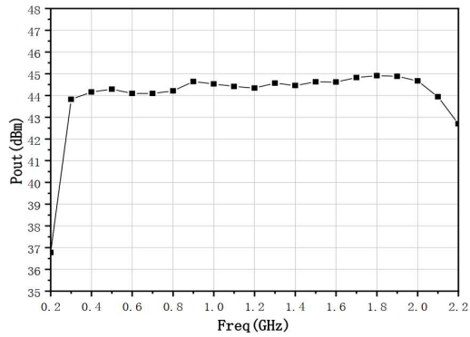
Output Power @ 48V
