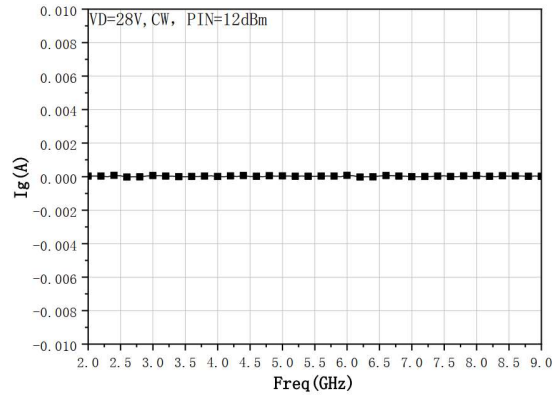
Grid Current vs. Freq
