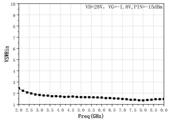
Input VSWR vs. Freq
