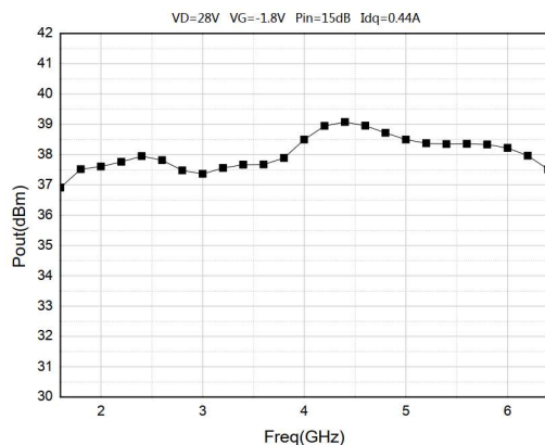
Output Power
