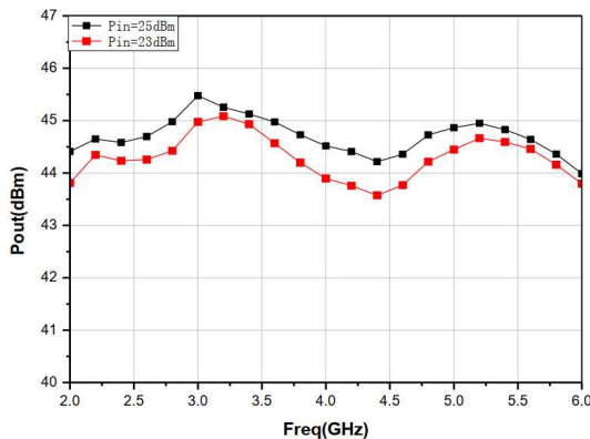
Output Power
