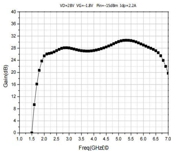
Small Signal Gain
