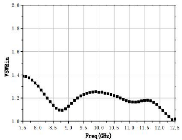
VSWR in
