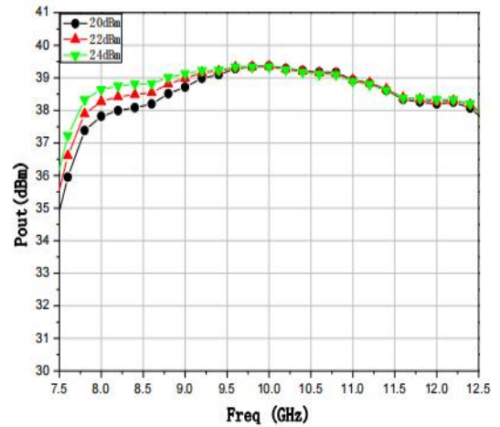
Pout@ Different Pin
