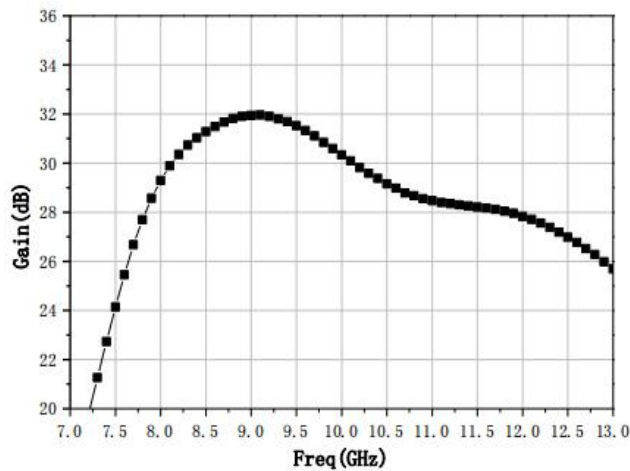
Small Signal Gain
