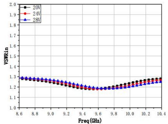
VSWRin@ Different Vd
