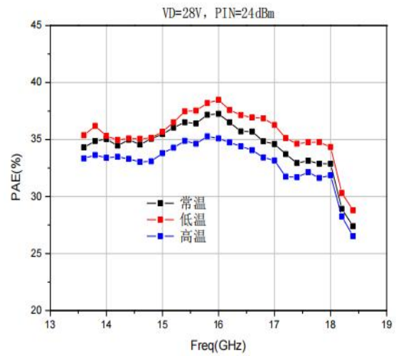
PAE @ Different Temp.
