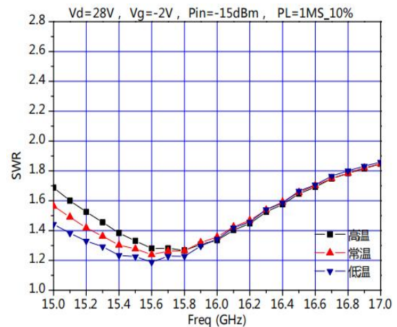
VSWRin@ Different Temp.
