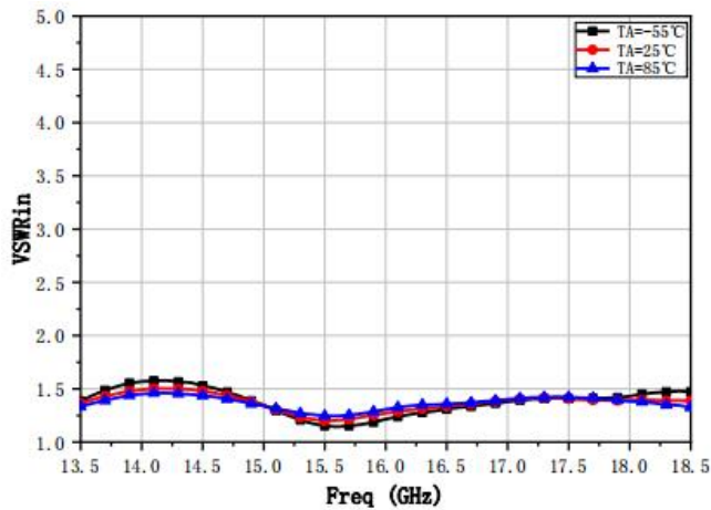
VSWR in @ Different Temp
