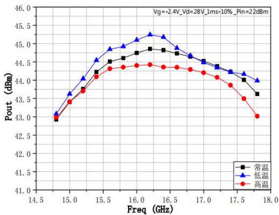
Pout@ Different Temp
