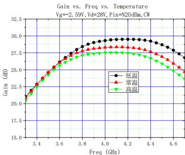
Small Signal Gain@ Different Temp
