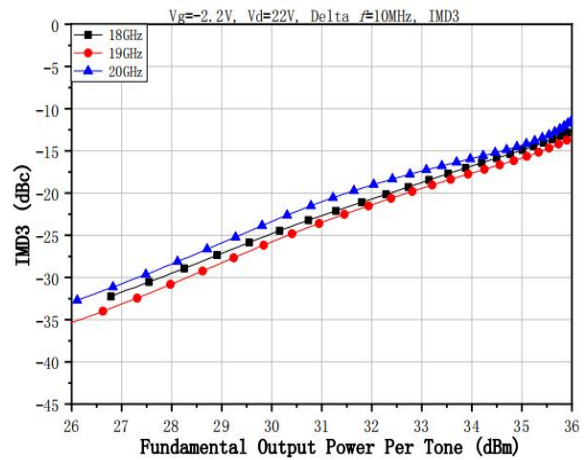
IMD3 VS pout/per tone
