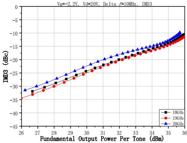
IMD3 VS pout/per tone
