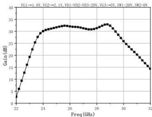
Gain
