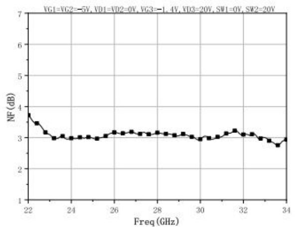
Noise Figure
