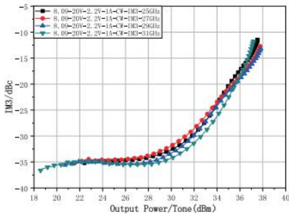
IM3 VS pout/per tone
