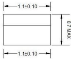
side view(left)
